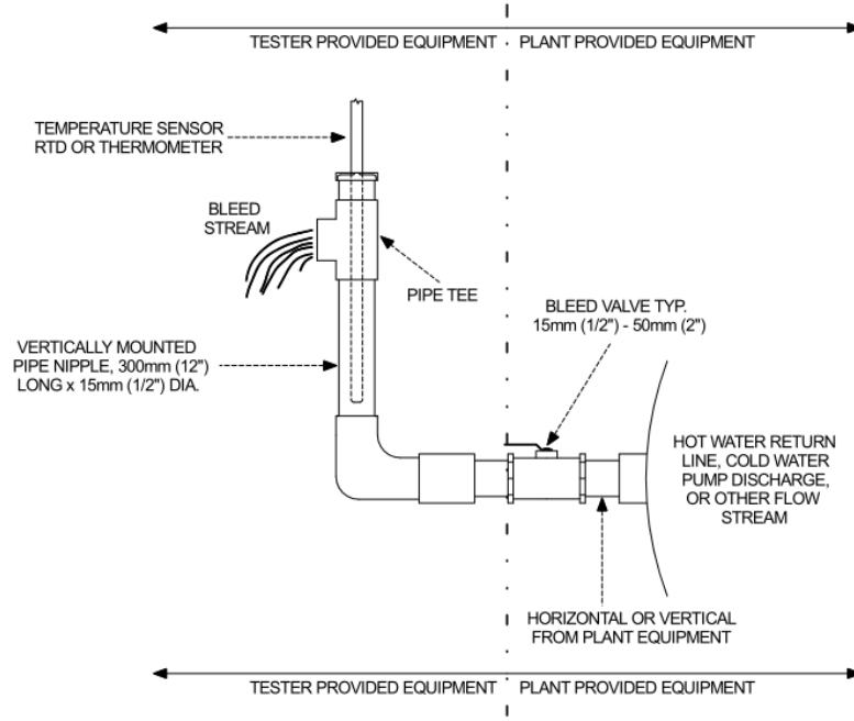
Figure 5: Temperature Tap Details
