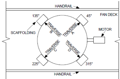
Figure 7: Scaffolding Requirements for Plume Abatement or Drift Testing
