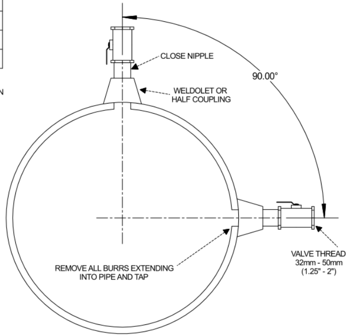
Figure 3: Pitot Tap Details (Section A-A from Fig. 1 & 2)
