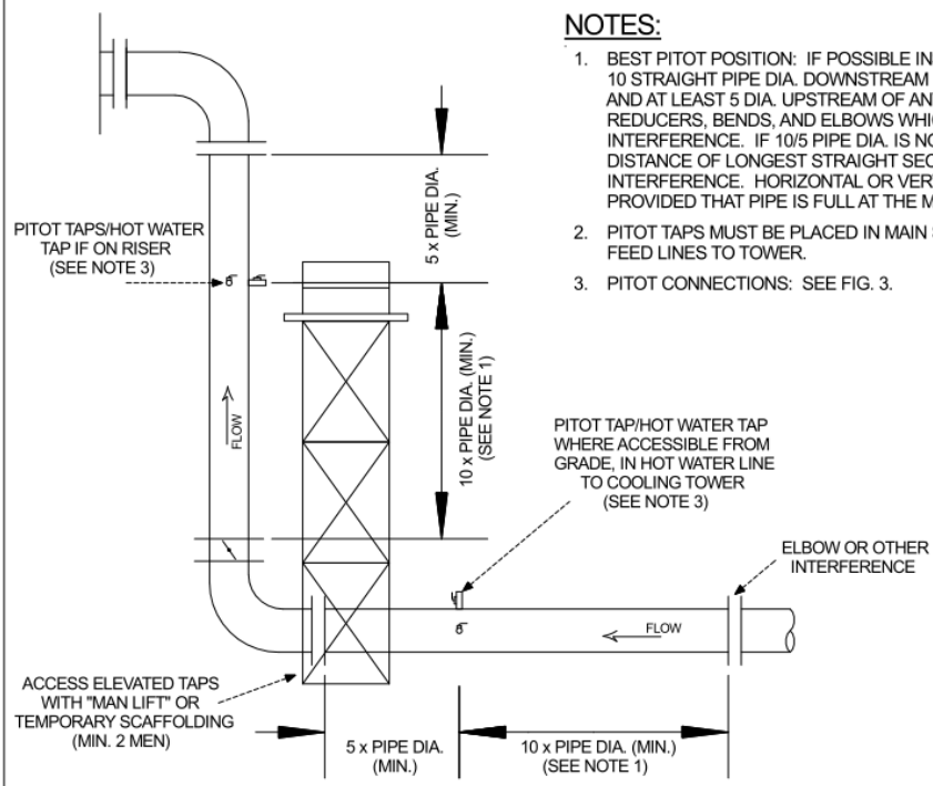
Figure 6: Typical Pitot Locations
