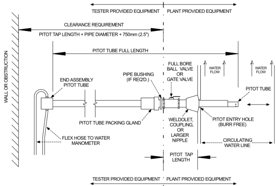
Figure 4: Pitot Tube Installation
