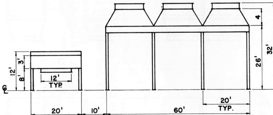
Figure 11 End elevation of air coolers installed in Canadian refinery. Hot air recirculated from air cooler at lower elevation.
