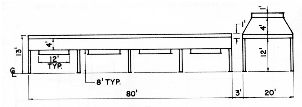
Figure 10 End elevation of air cooler layout in a southwestern natural gasoline plant. Hot air recirculation occurred where new induced draft air cooler was added to existing forced draft air cooler bank as shown.
