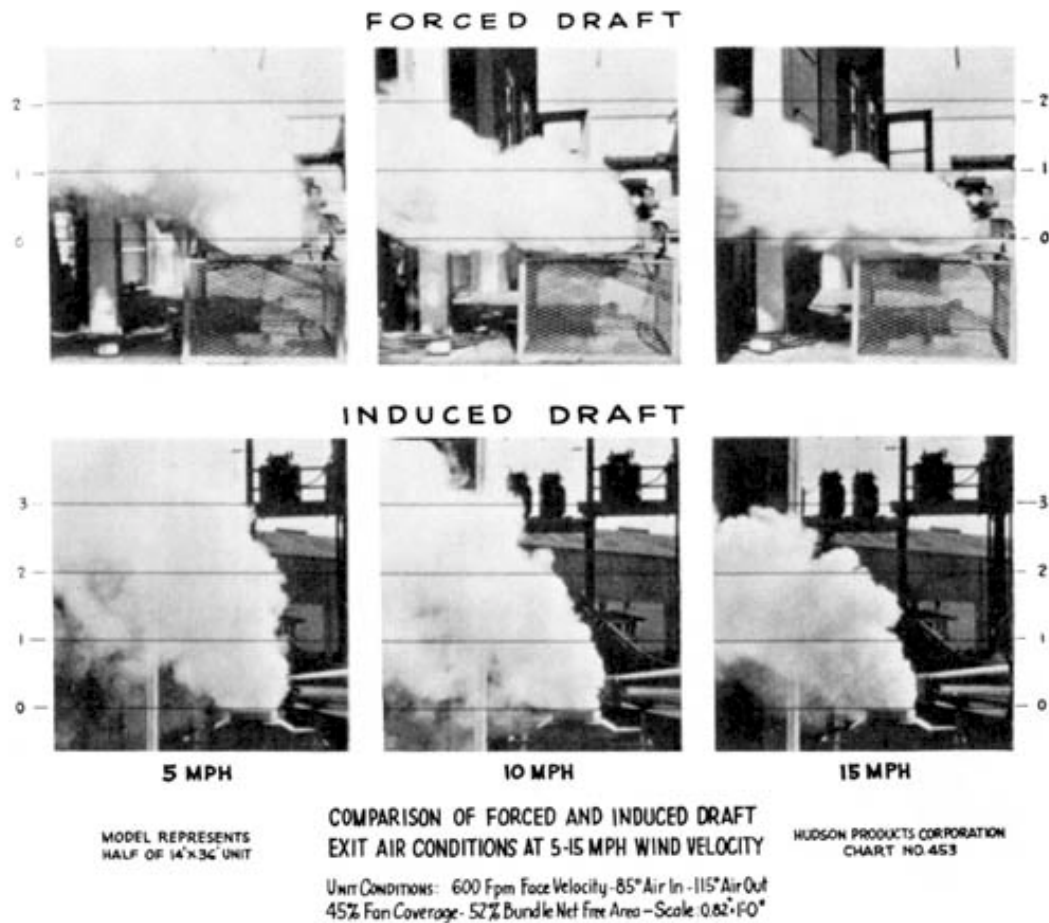
Figure 2 Comparison of forced and induced draft exit air conditions at 5-15 mph wind velocity; unit conditions: 600 fpm face velocity - 85° air in - 115° air out, 45% fan coverage, 52% bundle net free area - scale: 0.82" = 1' - 0"; Model represents half of 14' x 36' unit.
