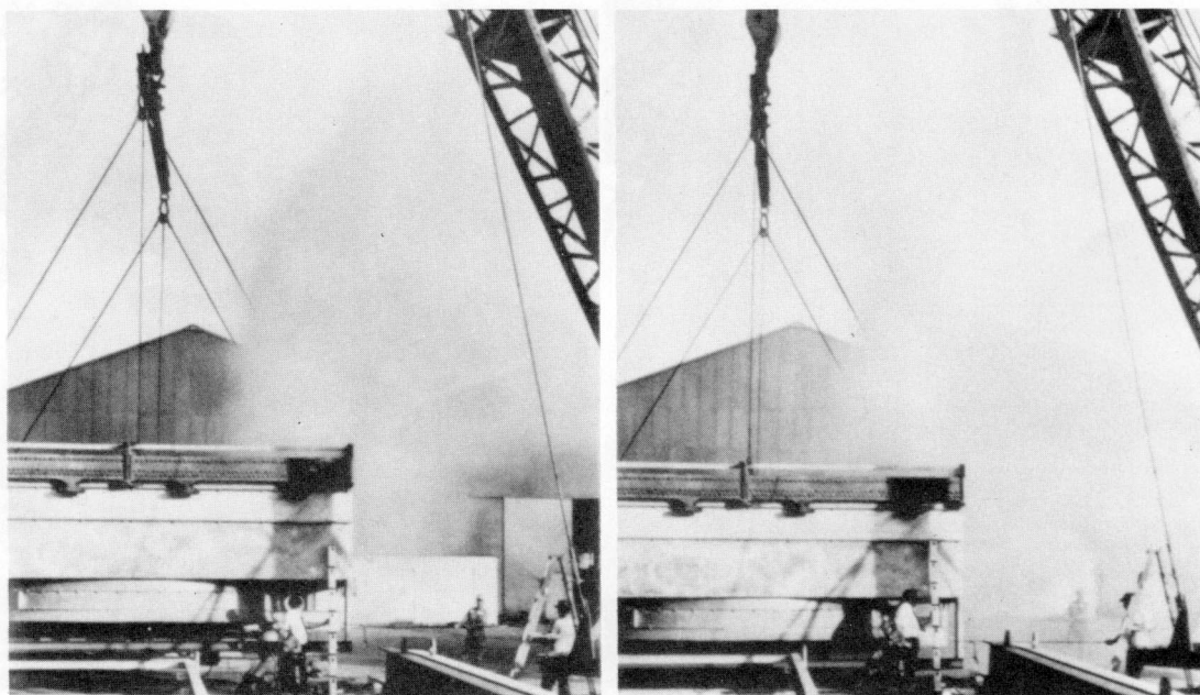
Figure 7C Smoke test on suspended air cooler at V_a = 7.5 and V_e = 8.1 , note some recirculation.
