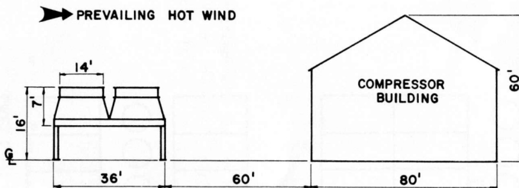
Figure 13 Jacket water coolers installed on gas pipelines near compressor building. Hot air recirculation due to building obstruction.
