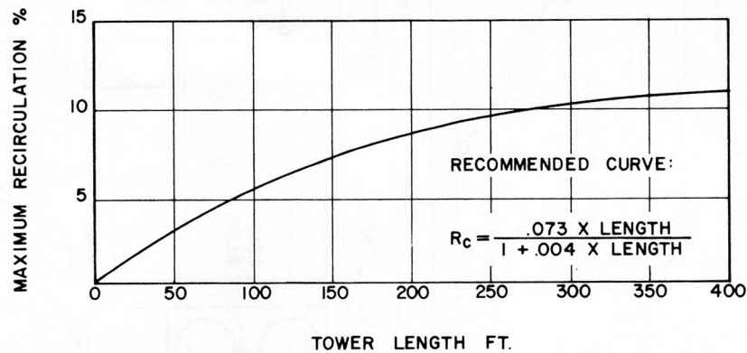
Figure 6 Maximum percent recirculation versus cooling tower length. Induced draft cooling towers only.
