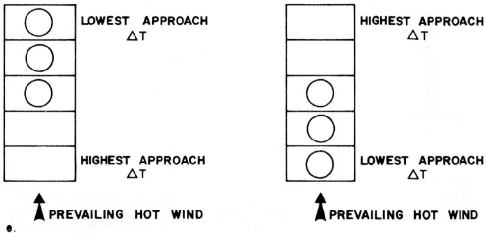
Figure 14(d)(e) Incorrect and correct air cooler layouts.
