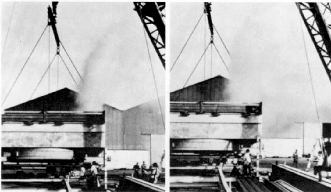
Figure 7A Smoke test on suspended air cooler at V_a = 6.1 and V_e = 8.1 , no recirculation.
