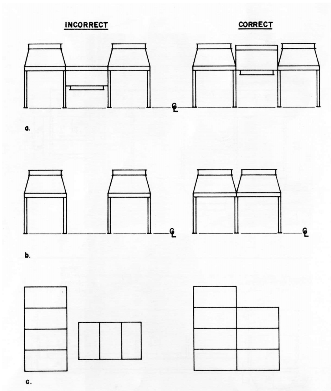
Figure 14(a)(b)(c) Incorrect and correct air cooler layouts.
